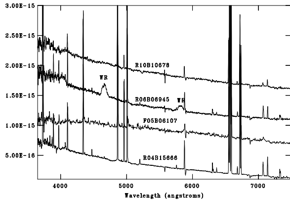
Fig. 1. Extracted spectra of 4 compact stellar clusters. The fluxes are in units of \text{erg cm}^{-2} \text{s}^{-1} \text{\AA}^{-1} . The fluxes of the top 3 spectra are displaced upwards for the sake of clarity.
