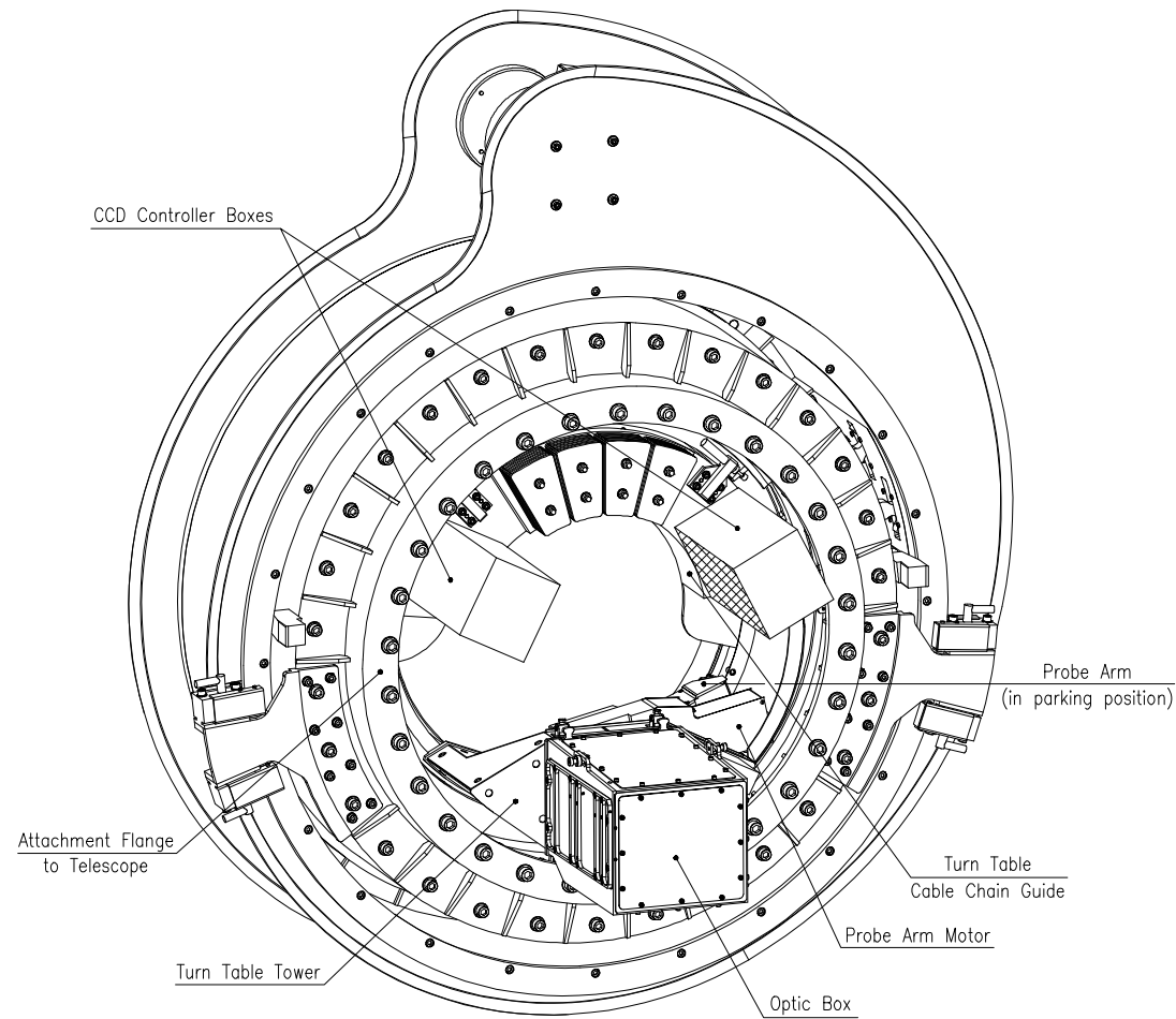
Lateral back view of the Folded Cassegrain Rotator
