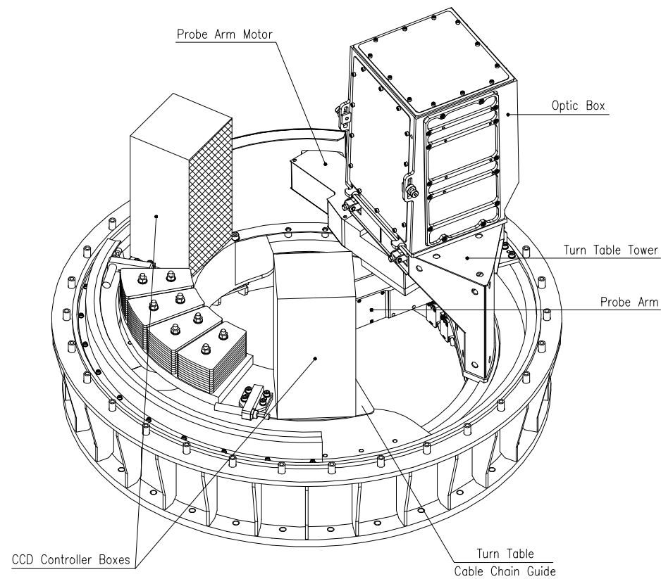
View of the inner Rotating Structure
