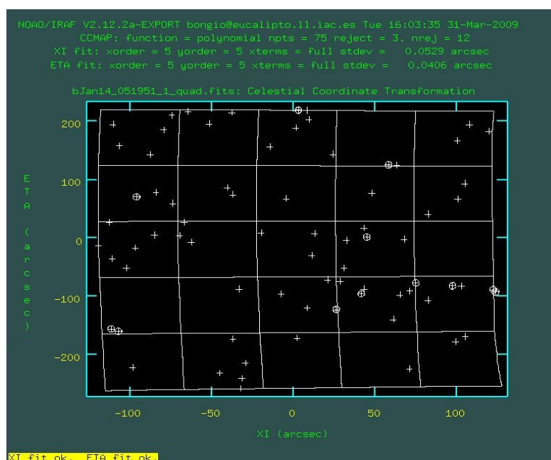
Figure 9.2.- Example of the IRAF task ccmap solution.
