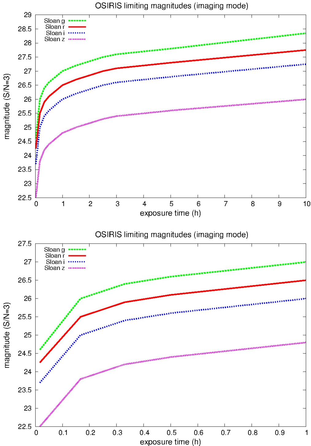
Figure 2.5.- Limiting magnitudes ( S/N=3 ) achieved with OSIRIS broad band filters as a function of the exposure time, assuming dark conditions, seeing = 1.0 arcsec, and airmass = 1.2. A detailed view for exposure times lower than 1.0 h is shown in the graph below.
