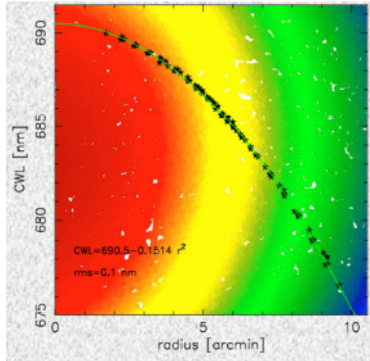
Figure 4.2.- Central wavelength variation along the OSIRIS FOV for SHARD filter U687/17, showing the radial variation along the optical centre (X_0, Y_0) for this filter that can be fitted by Equation 4.1.
