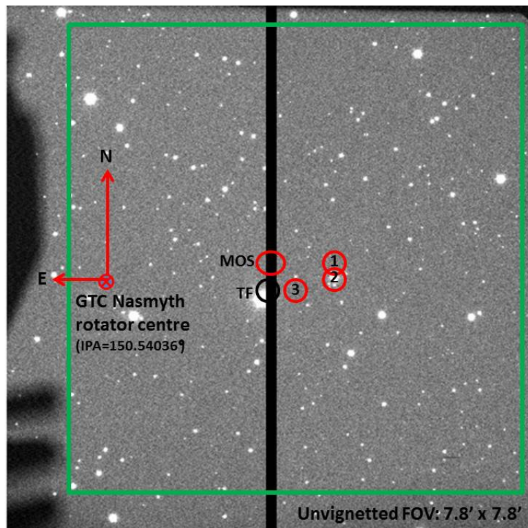
Figure 1.4.- OSIRIS image showing the shadowing produced by the folder flat and filter wheels on one side of CCD1 (left). Since the instrument is off-axis, the centre of the OSIRIS field does not coincide with GTC pointing centre
