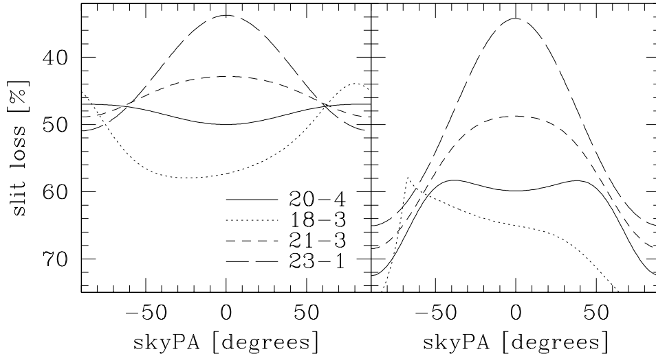
Fig. 5. Average slit loss at 4500 Å at different slit orientations. I used our sample observation of the Lockman Hole using Keck (see Sect. 1 for details – left panel ) and a southern field (CDFs, -27:48:30 declination – right panel ). I show the effect of slit sky position angle at different hour angle ranges. For sky position angle I use the (unusual) DEIMOS definition, where 90 degree is E-W, 0 degree is N-S.
